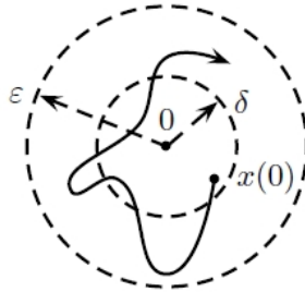
Figure 5.1 Stable equilibrium
