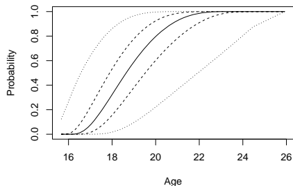
Population prior
